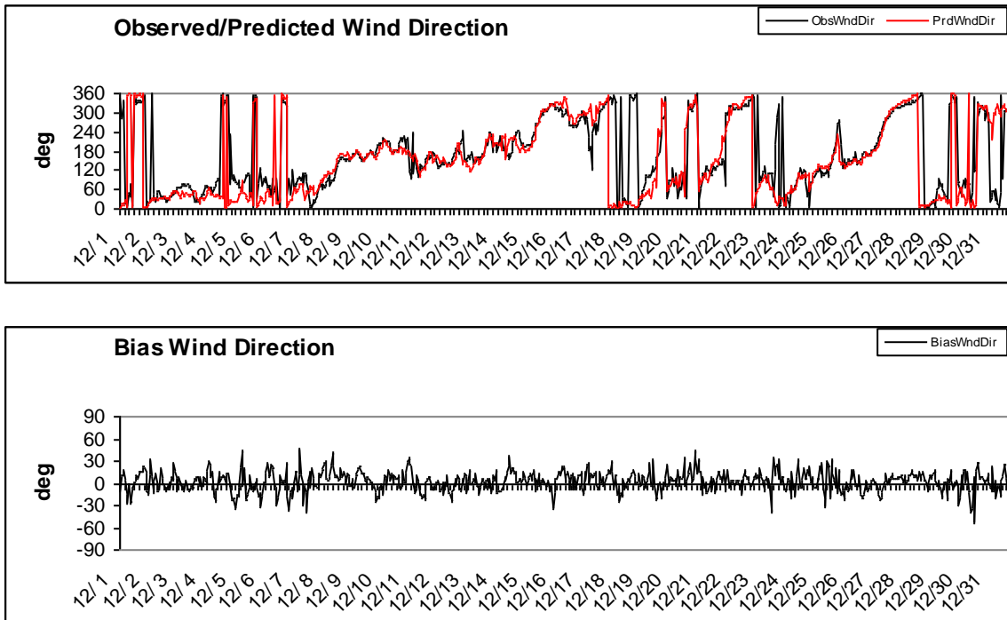
Figure B-10. Hourly time series of region-average observed and predicted surface-layer wind direction and performance statistics in the 4-km MM5 domain for December 2006.
