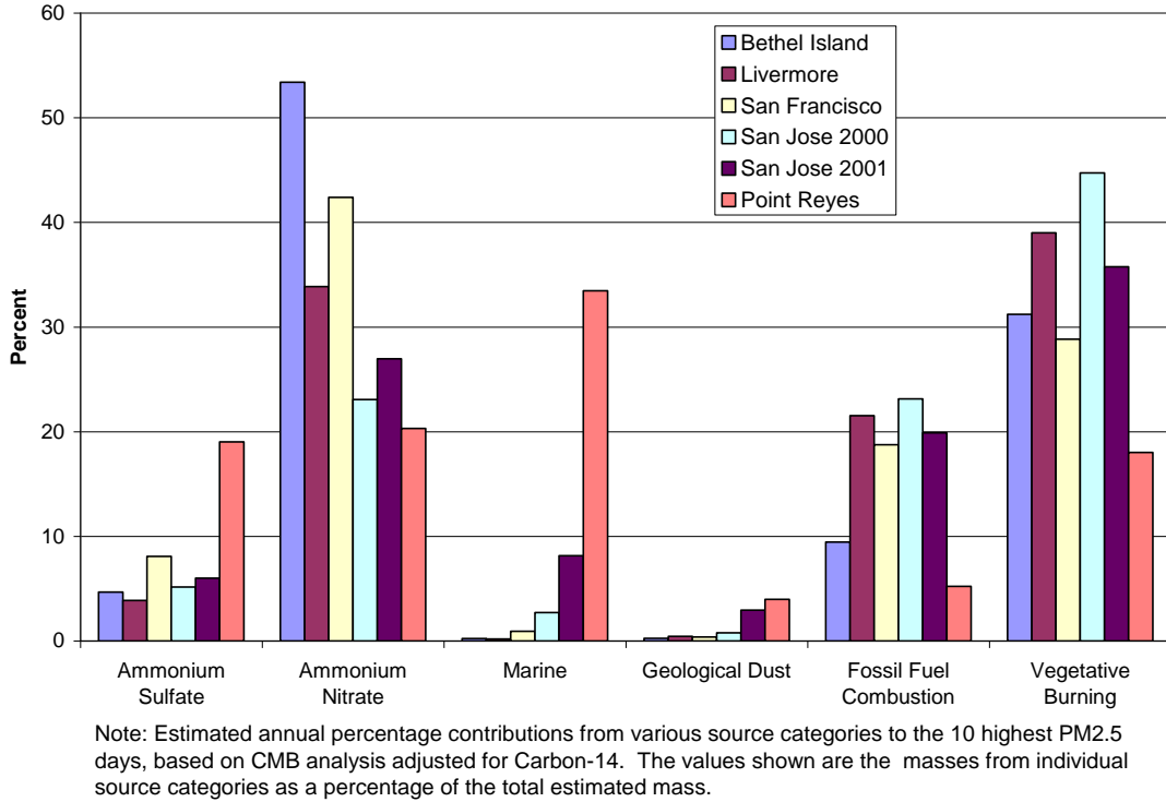
Figure 11. CMB results for CRPAQS period. Results for exceedance days only.
