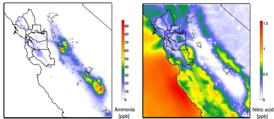
Figure 17. Aerial plots of simulated 24-hour levels for gas phase ammonia and nitric acid, averaged across the 55 days for which simulated Bay Area maximum 24-hour PM_{2.5} level exceeded 35 \mu\text{g}/\text{m}^3 . Bay Area counties and the California coastline are drawn using thick black lines. City limits for Sacramento, Stockton, Modesto, Fresno, and Bakersfield (listed north to south) are drawn using thin black lines.
