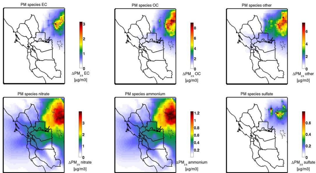
Figure 26. Benefit ( \Delta PM_{2.5} ) upon eliminating anthropogenic emissions for the Sacramento area. Averaged across same 55 days as for Figure 16 having base case simulated Bay Area PM levels exceeding 35 \mu g/m^3 .
