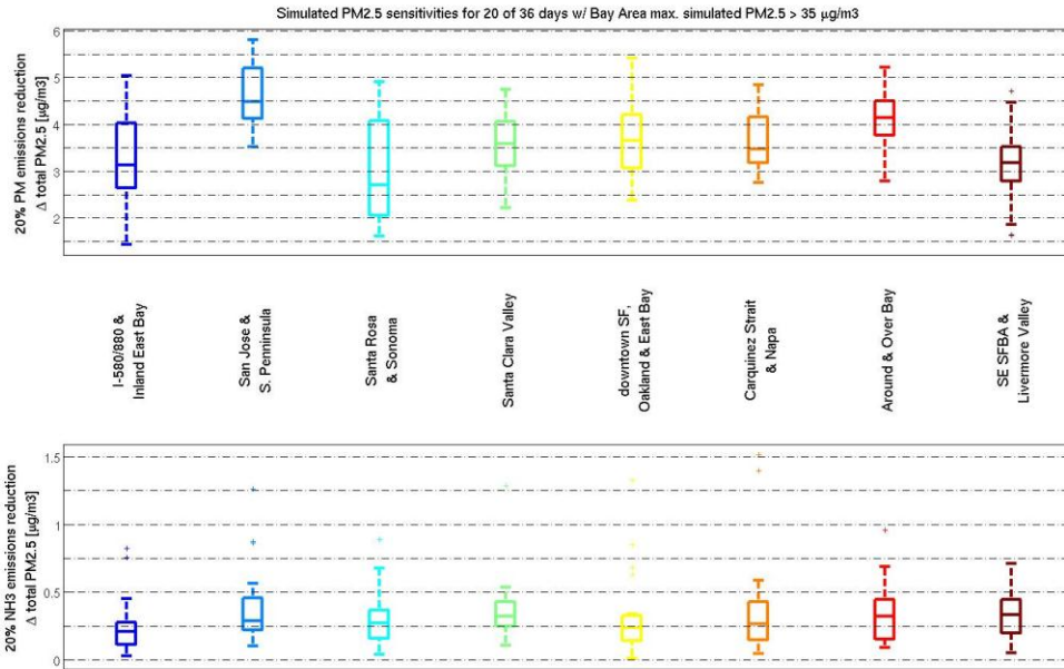
Figure 22. Tabulated \Delta PM_{2.5} values for grid cell with highest simulated PM_{2.5} level for eight subdomains depicted in Figure 18, for 20 exceedance days only. Top plot shows sensitivity to 20% direct PM emissions reductions. Bottom plot shows sensitivity to 20% ammonia reductions. Horizontal lines on boxes indicate 25 th , 50 th (median), and 75 th percentiles for \Delta PM_{2.5} values. Remaining values are contained within whiskers, except for outliers plotted using a plus signs.
