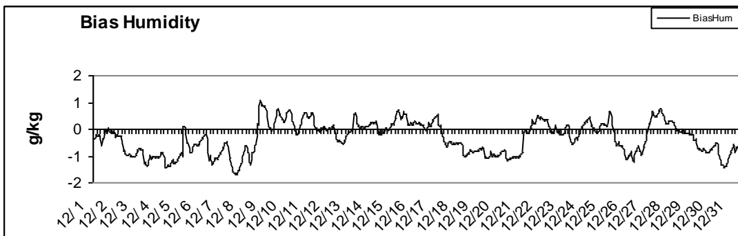
Figure B-12. Hourly time series of region-average observed and predicted surface-layer humidity and performance statistics in the 4-km MM5 domain for December 2006.
