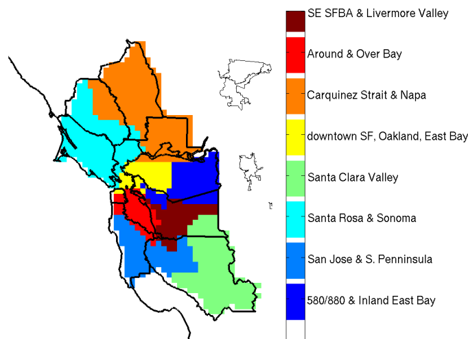
Figure 18. Eight Bay Area subdomains sharing similar air quality characteristics when PM levels are elevated. Bay Area counties and the California coastline are drawn using thick black lines. City limits for Sacramento and Stockton are drawn using thin black lines.
