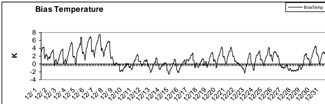
Figure B-11. Hourly time series of region-average observed and predicted surface-layer temperature and performance statistics in the 4-km MM5 domain for December 2006.
