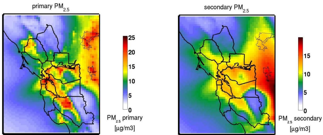
Figure E-1. Spatial distribution of simulated primary and secondary PM 2.5 levels, averaged across the 52 simulated days for which measured Bay Area 24-hour PM 2.5 level exceeded 35 µg/m 3 . Bay Area counties and the California coastline are drawn using thick black lines. City limits for Sacramento and Stockton are drawn using thin black lines.
