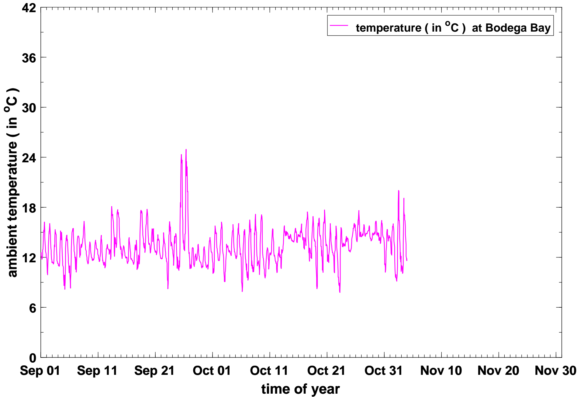
Timeseries of hourly-averaged air temperatures (in degree Celsius) at Bodega Bay during fall 2016 (Sep 1 - Nov 30).
