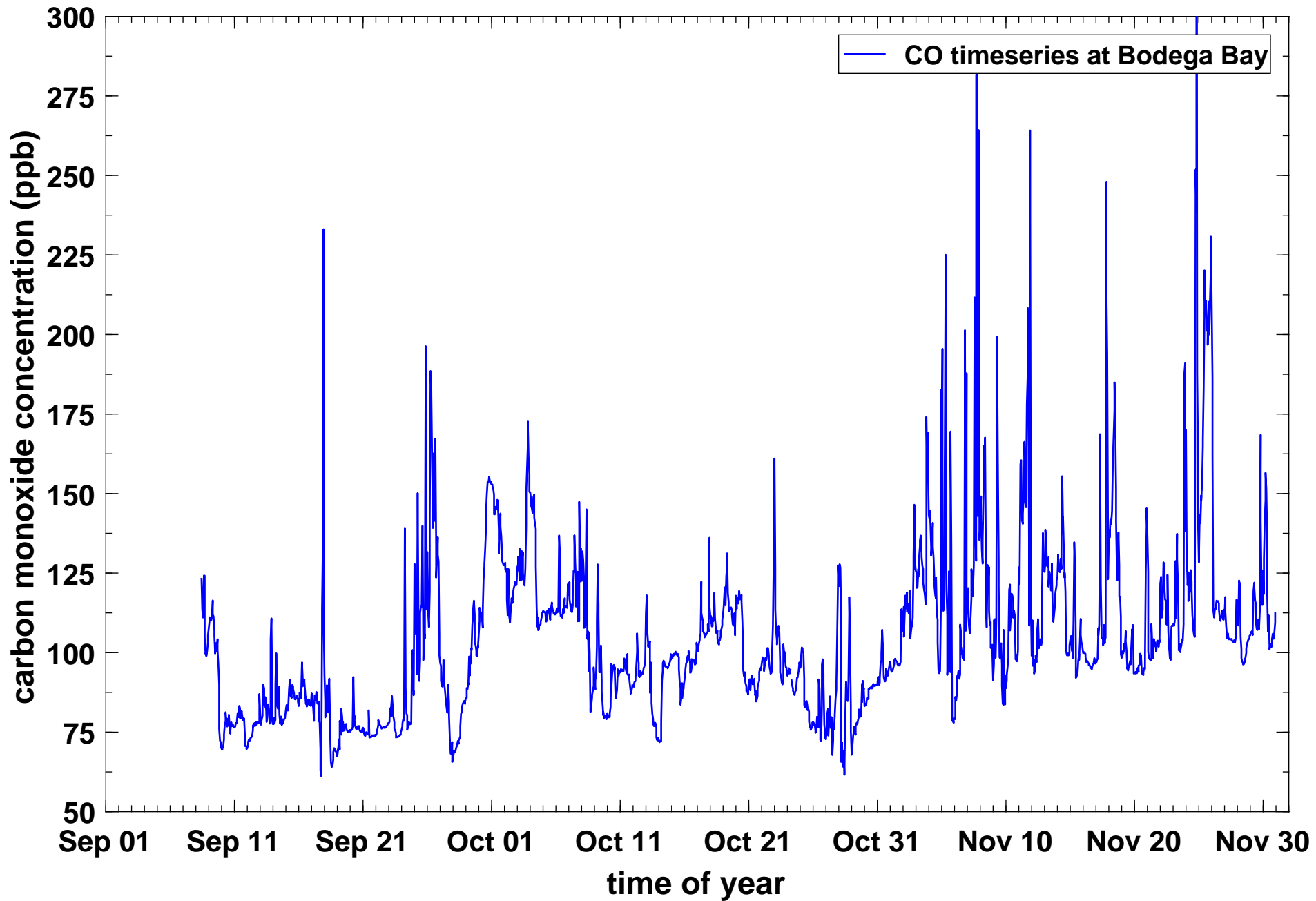
Timeseries of hourly CO concentrations (in ppb) at Bodega Bay during fall 2016 (Sep 1 - Nov 30)..
