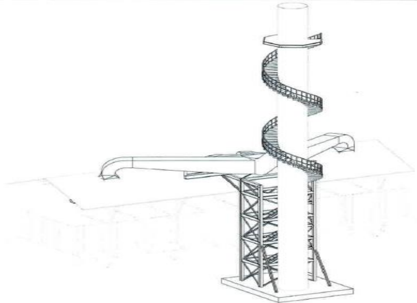
COOLER VENT SYSTEM REPLACEMENT 3D MODEL VIEW (LOOKING NORTHWEST) 4/9/2013
