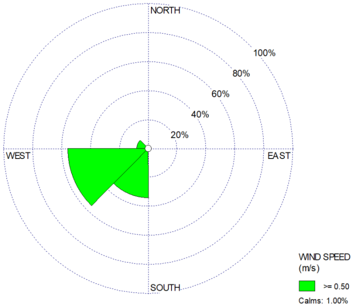
Figure 8 - Wind Rose - Summer Months (June, July, August: 2012 - 2016)
