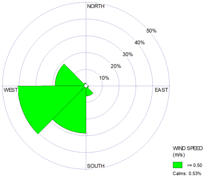
Figure 7 - Wind Rose - Spring Months (March, April, May: 2012 - 2016)
