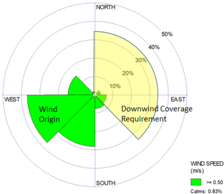
Figure 2 - Annual Wind Rose (SF1 Met Data Analysis January 1, 2012 - December 31, 2016)
