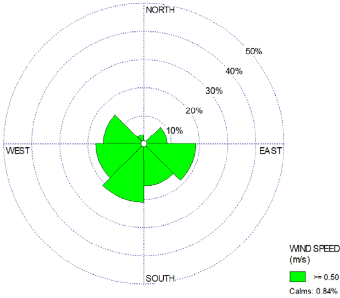
Figure 6 - Wind Rose - Winter Months (December, January, February: 2012-2016)
