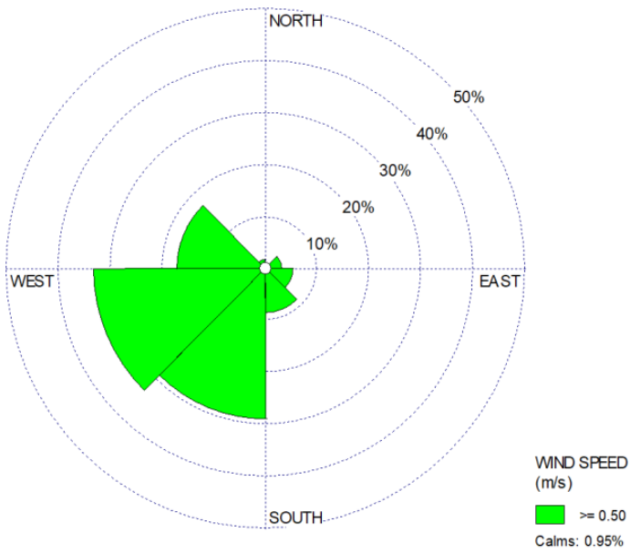
Figure 9 - Wind Rose - Fall Months (September, October, November: 2012 - 2016)
