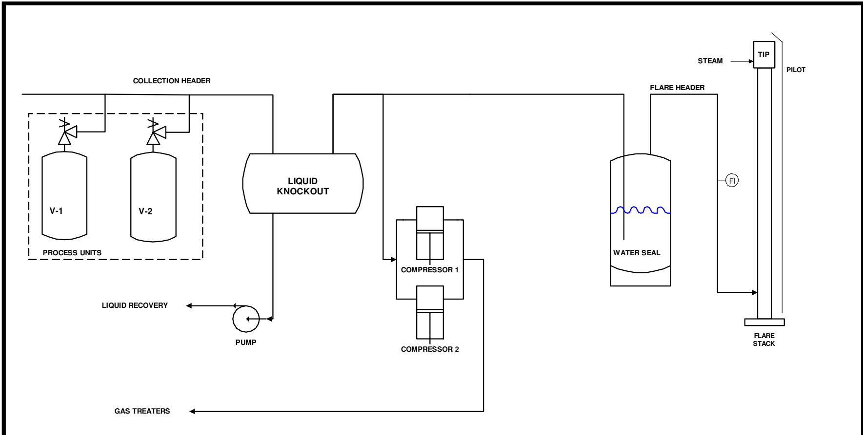
FIGURE 1. LOP AREA FLARE PROCESS SKETCH
