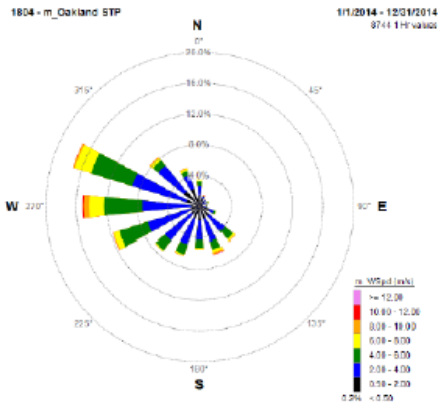
Figure 3-2. Annual windrose at the Oakland Sewage Treatment Plant (OST) in 2014. Compass sectors indicate the direction from which the wind is blowing. The percentage of calm winds (WSpd < 0.5 m/s) are also indicated.
